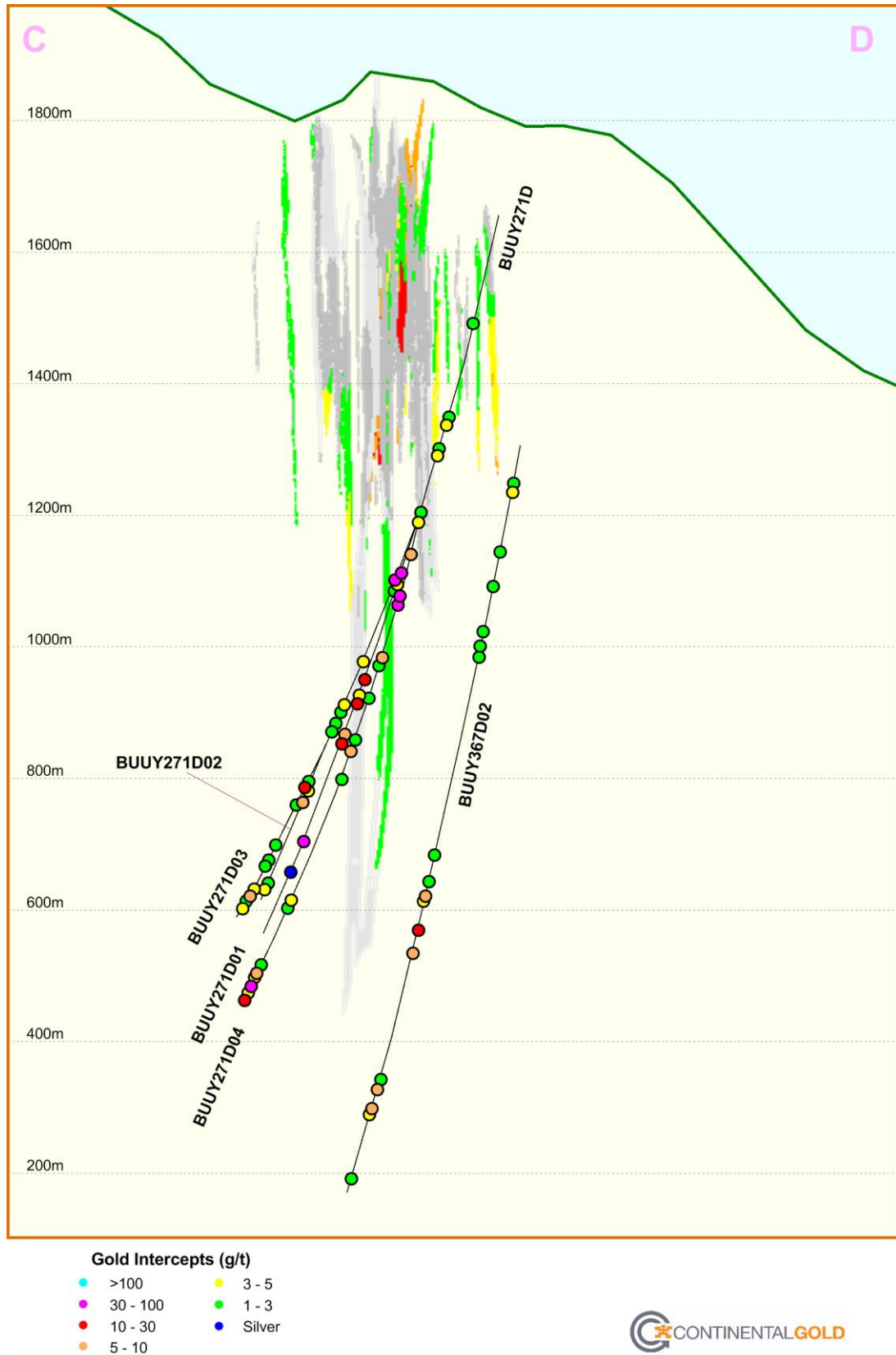
Figure 3 – Drill Section (Line C-D on Figure 1), showing highlights of new drilling (BUUY271D-series holes) against gold grades from the current Yaraguá and Veta Sur mineral resource block models
