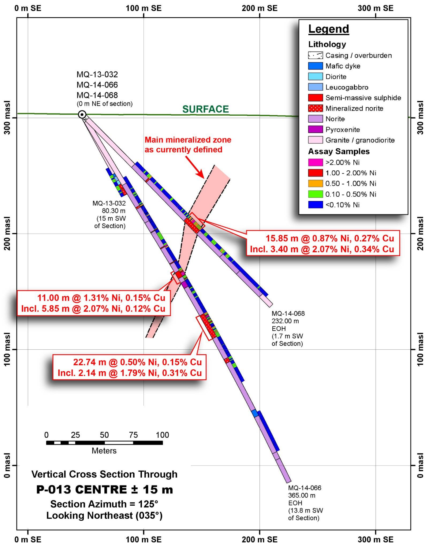
Figure 2: Vertical cross section through the P-013 Centre VTEM target. The section's azimuth is 125° and it looks 035° (northeast).
