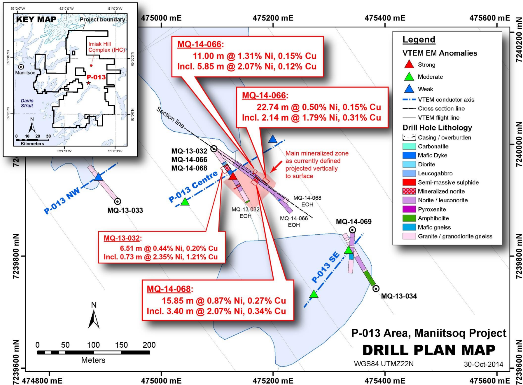
Figure 1: Plan map of the P-013 area with diamond drill holes projected to surface, VTEM EM conductors and significant assays.
