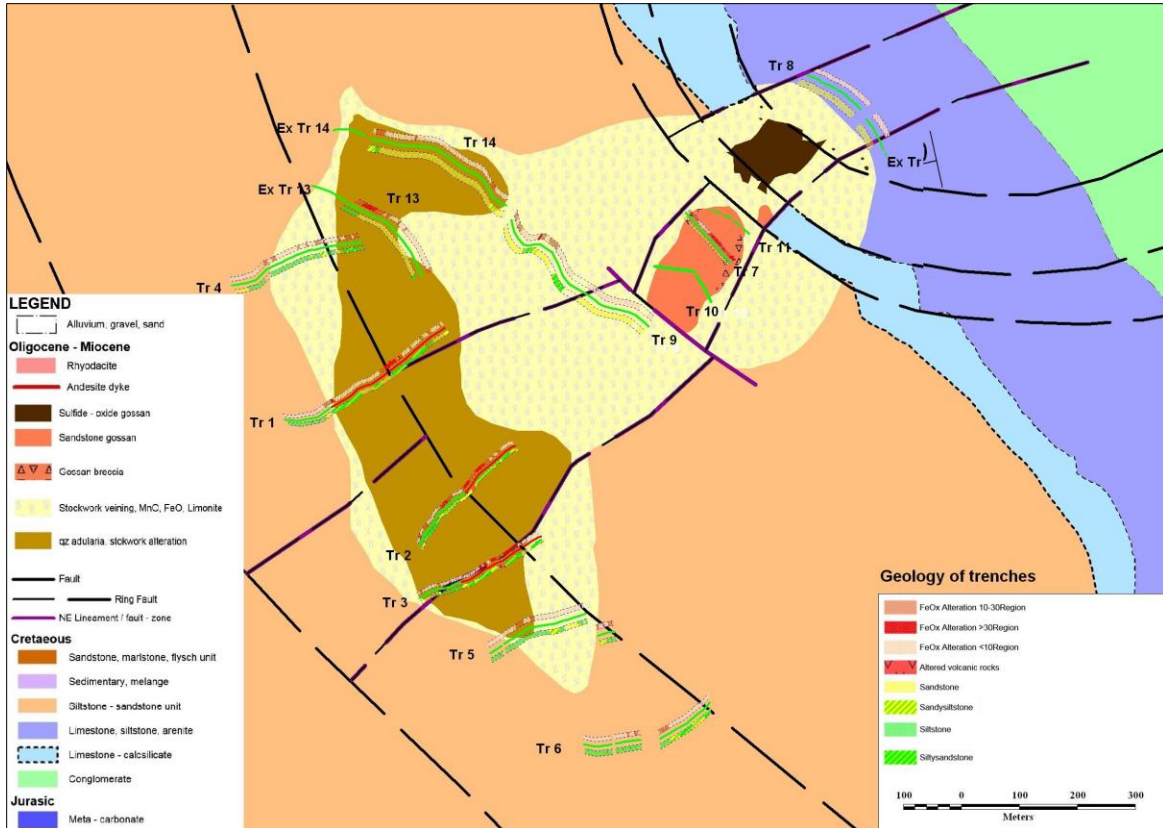
Figure 2. The Slivovo mineralization zone runs on the surface for over 1,000 meters along an ENE-trending corridor from the epithermal target ( olive ) to the SW gossan extension ( orange ) to the Pester sulfide-oxide gossan ( black ). The epithermal zone now runs for over 800 meters, north-south. Drilling started in the Pester gossan area and moved to the SW extension zone, where SLV008 is underway.
