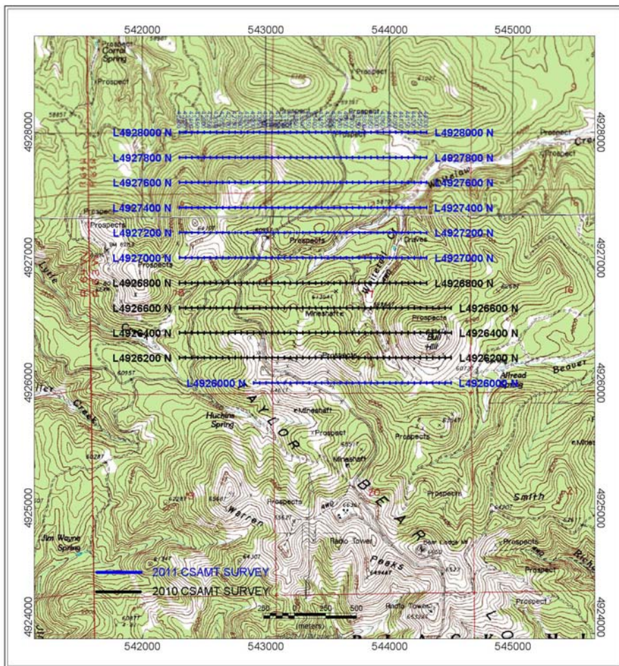
Figure 3. Location of CSAMT survey lines.
