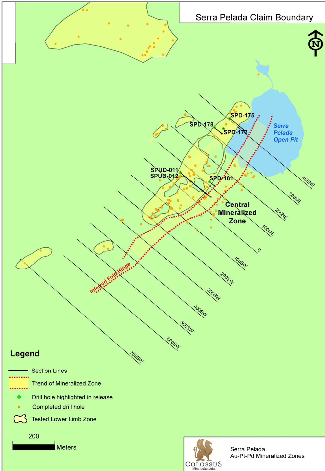
Figure 1: Plan View of Serra Pelada Mineralized Zones with location of reported holes. (Note: underground drill holes are projected to surface).
