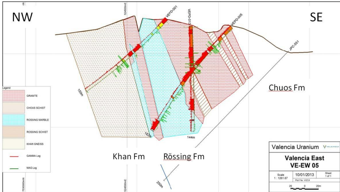
FIGURE 3. General structure of Valencia E with D-type alaskite intruding along Rössing Marble contacts.
