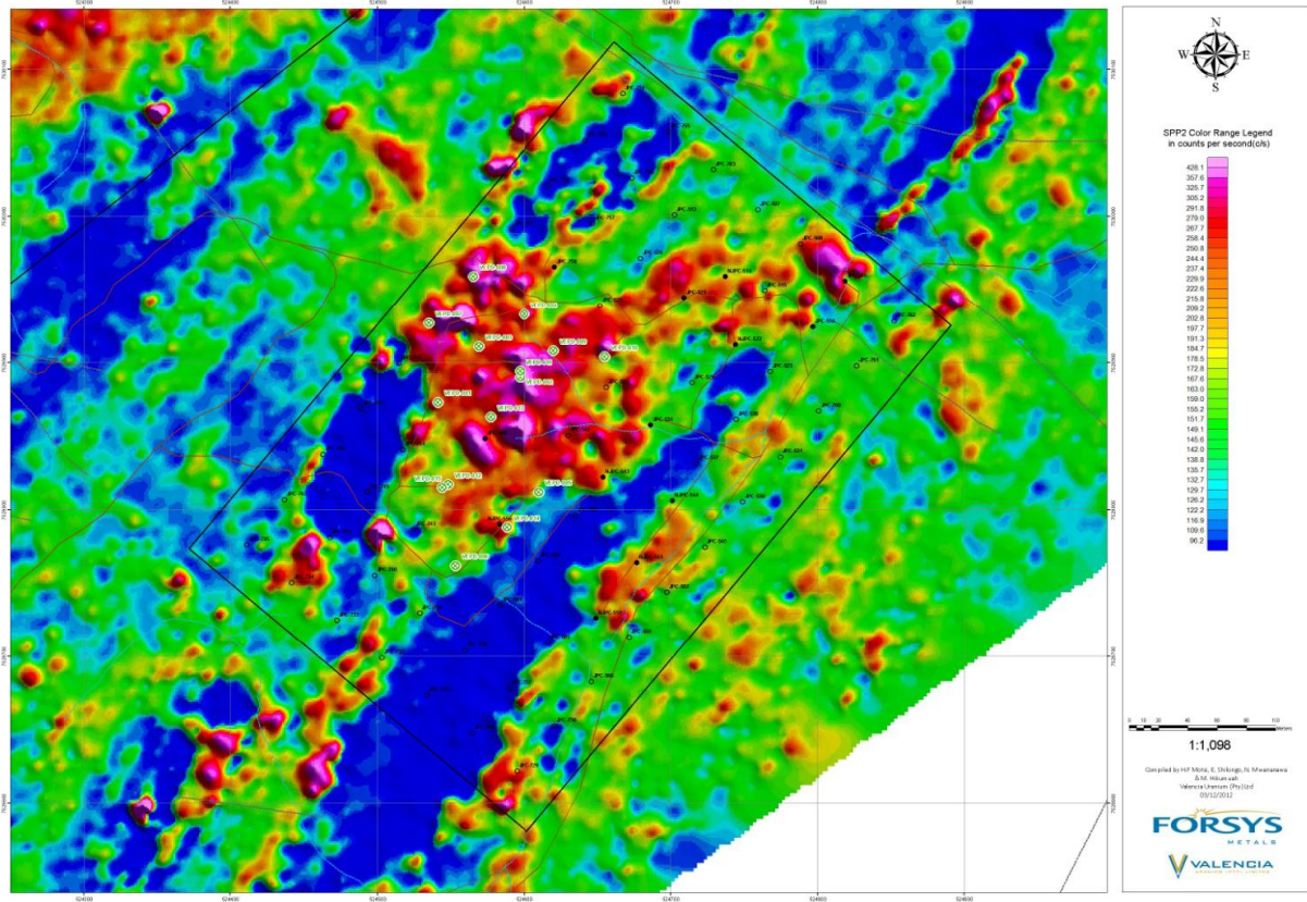
FIGURE 4. Radiometric footprint of the Valencia East area.
