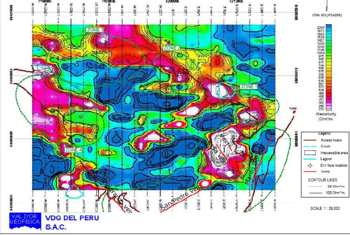
Figure 2. Lumpampa 2011 -- Induced Polarization Survey 3D Resistivity (Depth - 50 meters)
