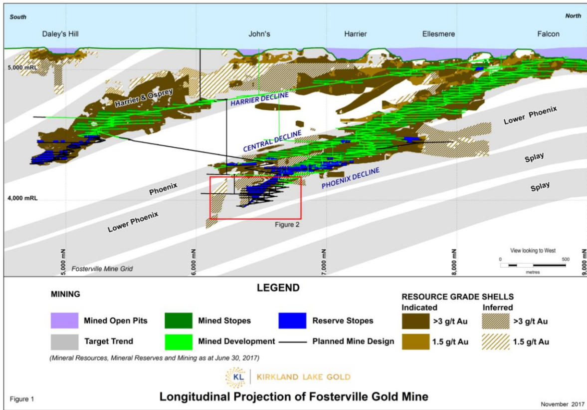
Figure 1. Long Section of Fosterville Gold Mine
