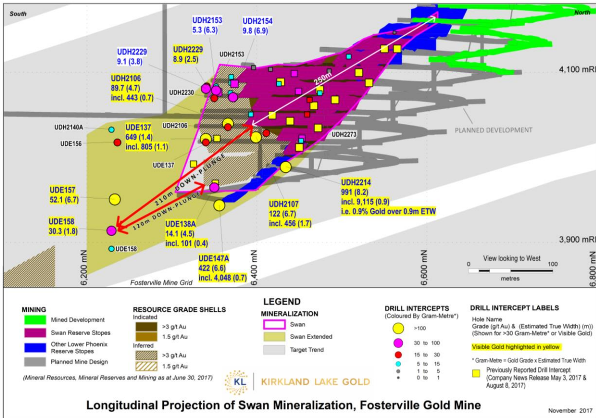
Figure 2. Long Section of Swan Zone
