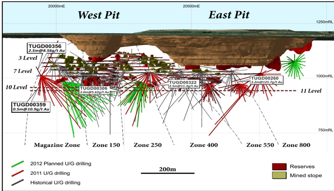
Figure – Tulawaka East Zone long section showing better intersections from drilling below 7Level
