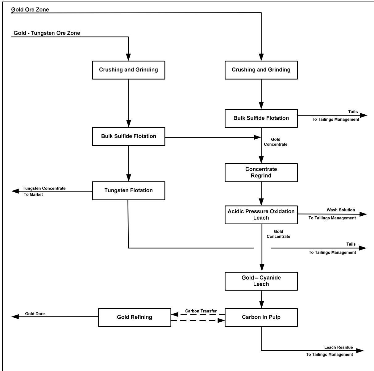
Figure 3: Block Diagram Overview of the Twins Lakes Process Technology
