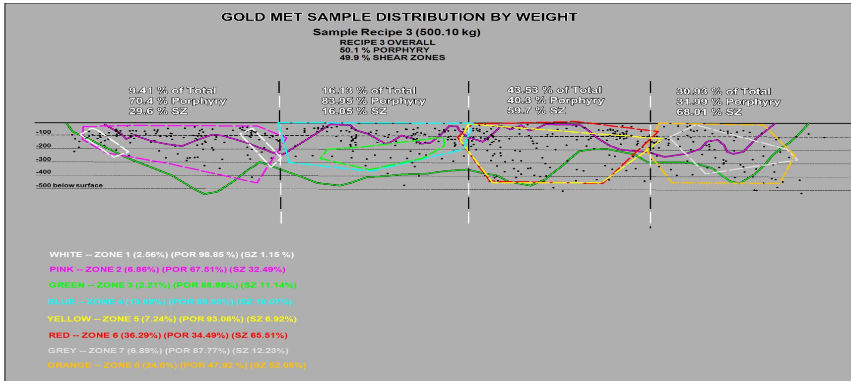
Figure 2: Long Section of the Twin Lakes Conceptual Pit Displaying Gold Metallurgy Sample Distribution by Weight
