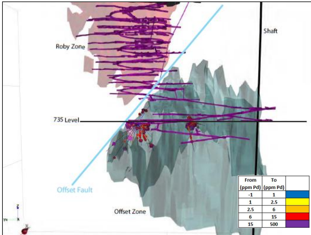
Figure 2: Offset Zone infill drilling on 15-m centre.
