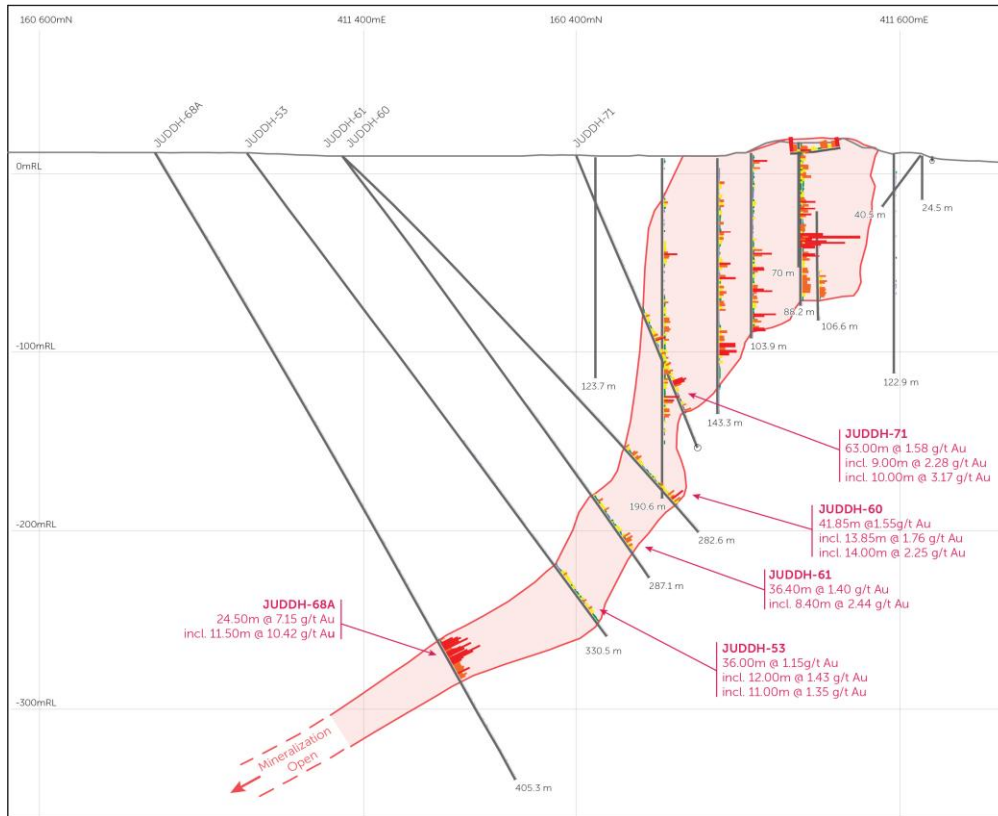
Bau Gold Project Jugan Hill Deposit Section Looking Northeast
