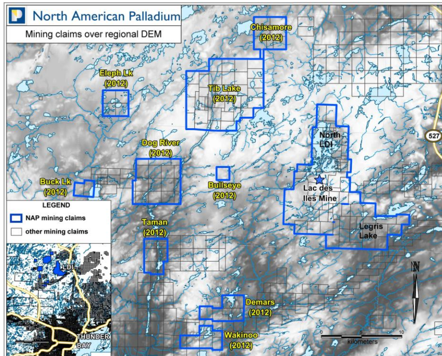
Figure 2: Location of NAP's Lac des Iles mine property and its Lac des Iles area greenfields PGE properties, Thunder Bay Mining District, northwestern Ontario. All of the greenfields properties are located within 30 kilometers of the LDI mill.
