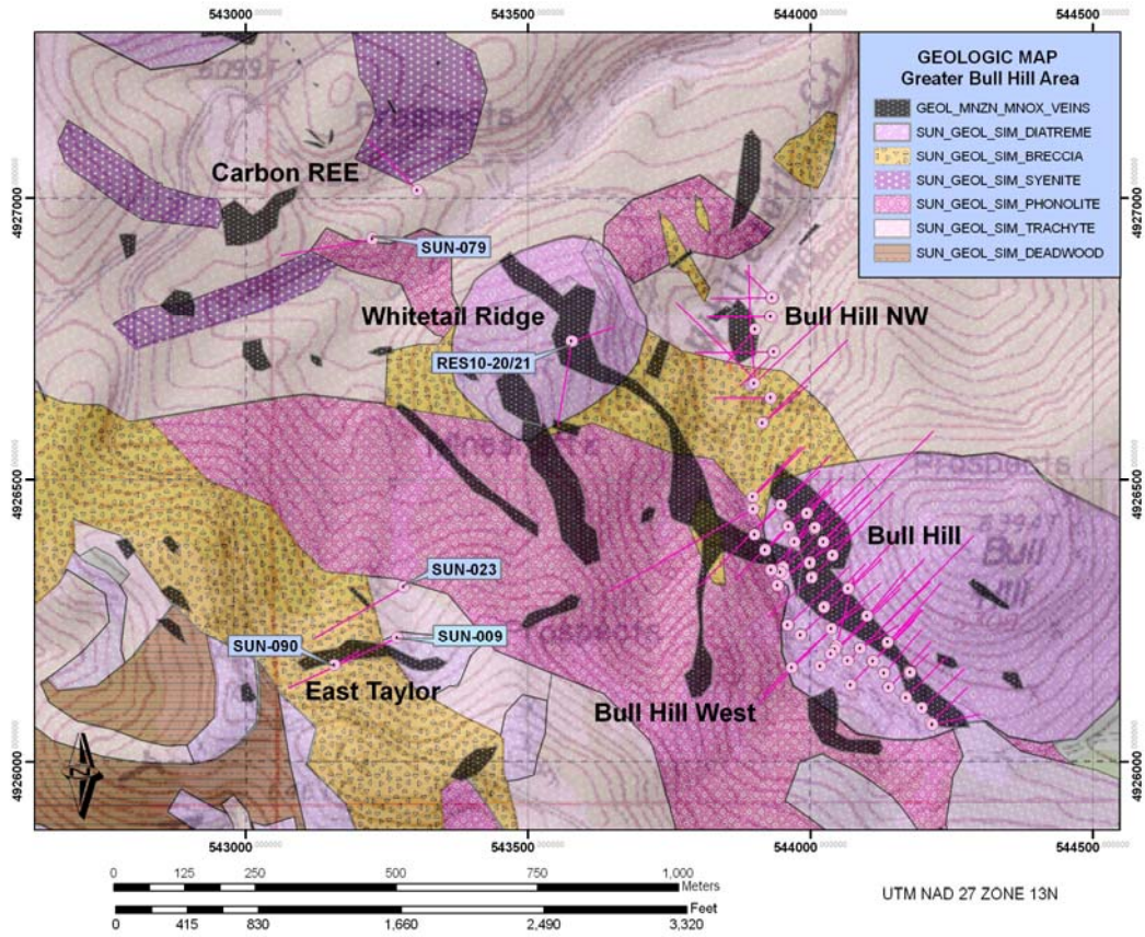
Figure 2. Bear Lodge REE district. The Whitetail Ridge resource area and the East Taylor and Carbon target areas are characterized by enrichments in HREE relative to REE abundances at the Bull Hill resource area.
