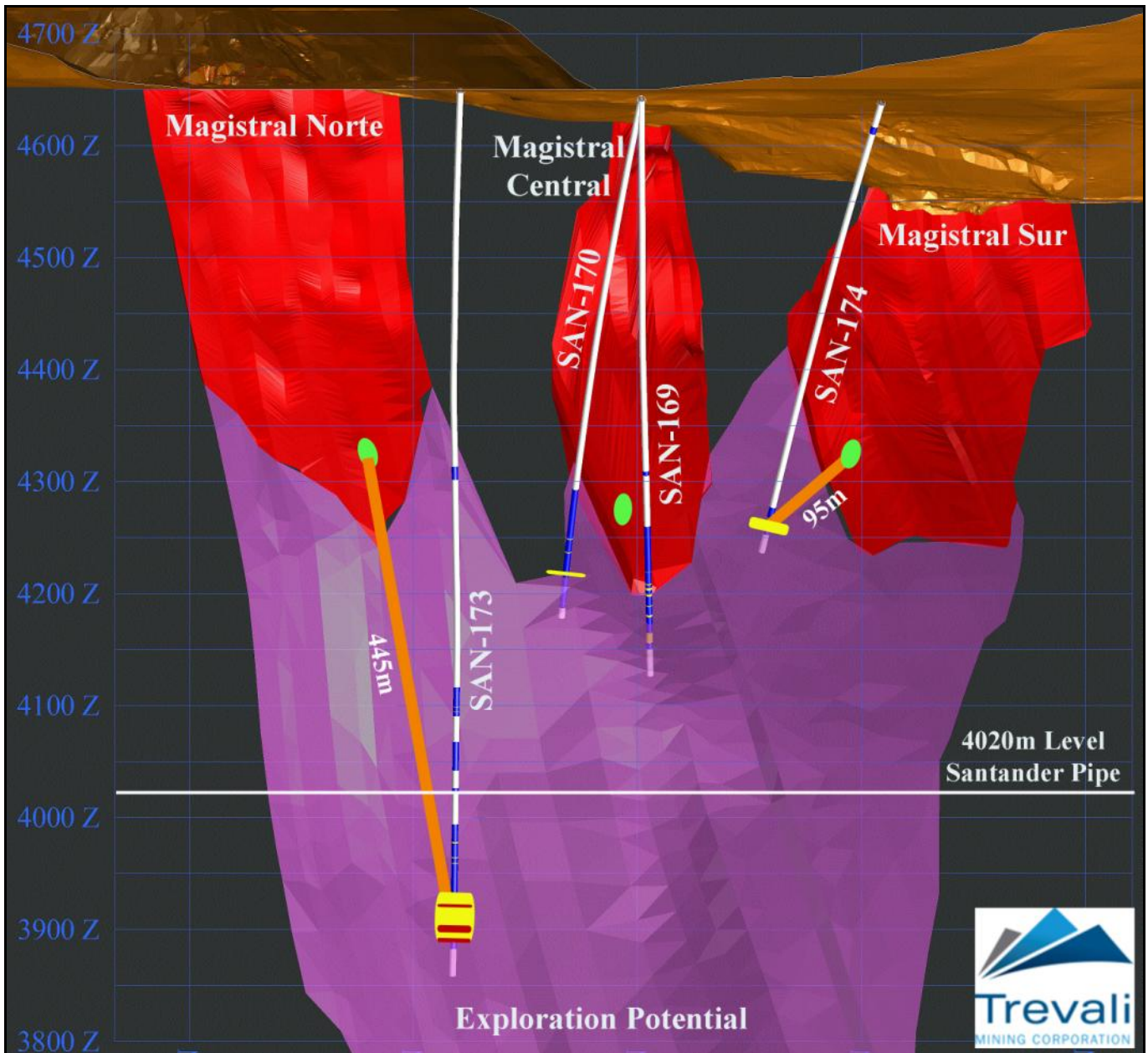
Figure 1: Long section looking east at the Magistral bodies and 2011 drilling. Green circles represent 2010 deepest drill hole intercepts. Purple surface represents exploration potential. The 4020-metre level of the Santander pipe represents the deepest level mined at the historic Santander Pipe operation.
