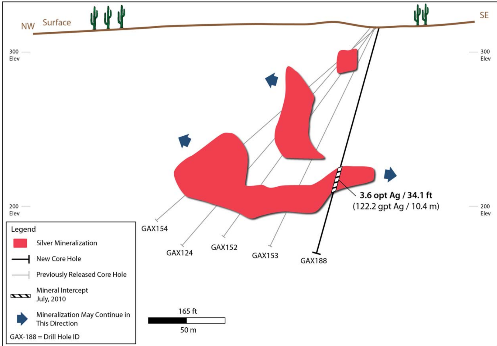
Figure 3 El Gallo Cross Section – Looking East (Section Number: NWSE South 26)
