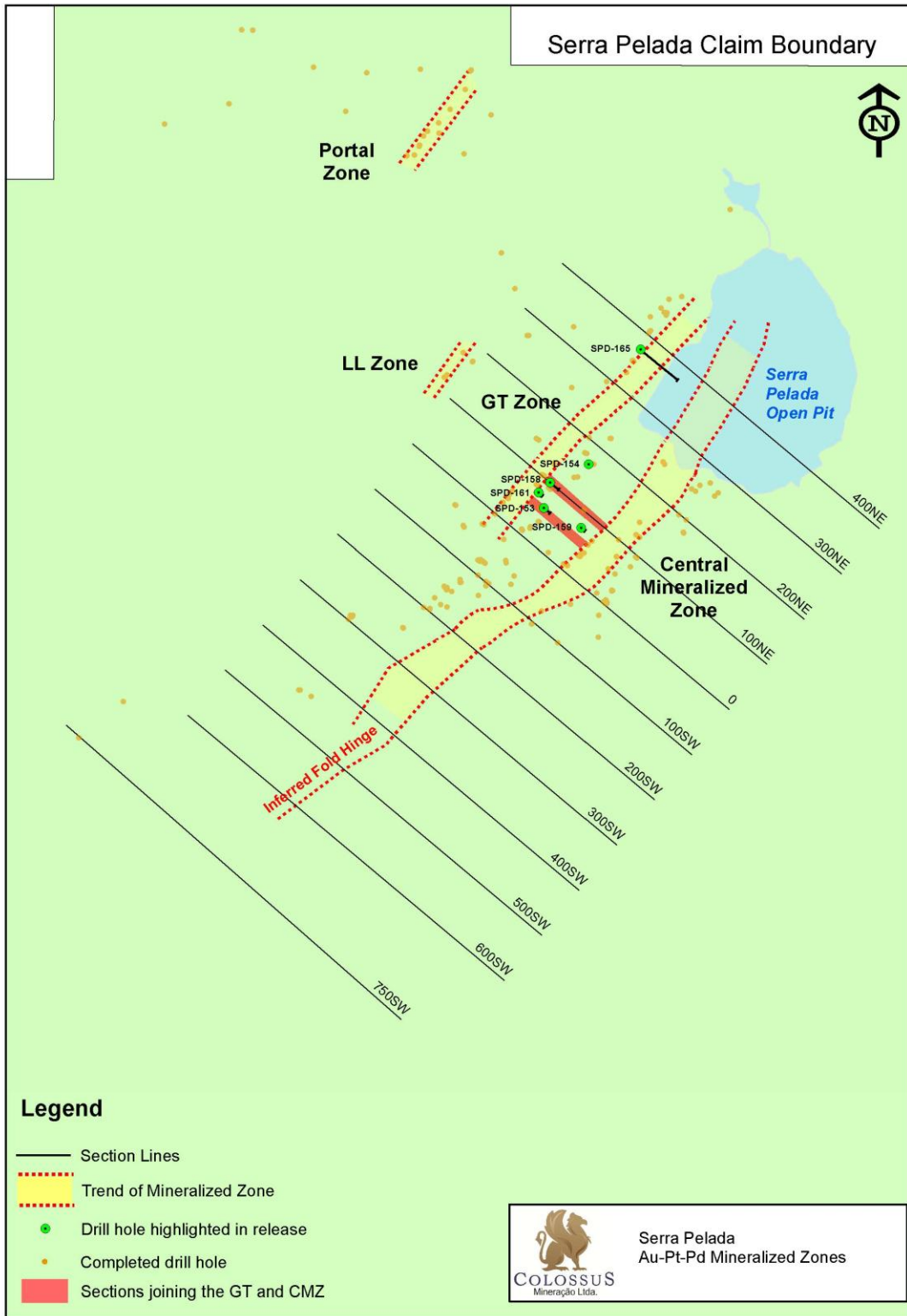
Figure 1: Plan View of Serra Pelada Mineralized Zones
