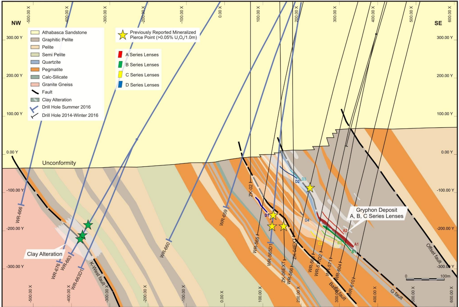
Figure 4: Cross-section along section line 5050 GP showing the intersection of mineralization and alteration at K-West in drill hole WR-663.
