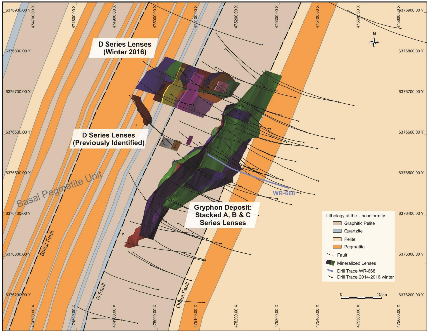
Figure 2: Plan map of the northeast plunging Gryphon mineralized lenses projected up to the simplified basement geology at the sub-Athabasca unconformity. The location of the first infill hole WR-668 is provided.
