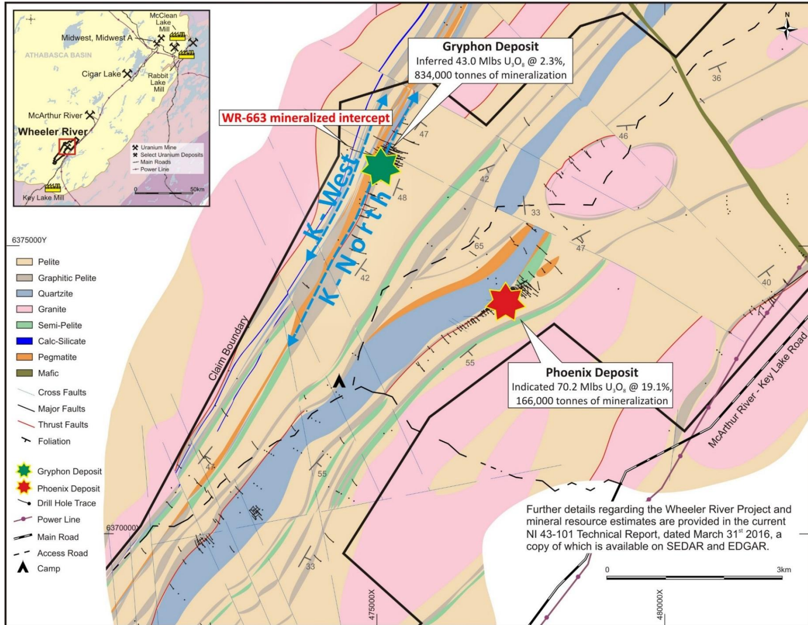
Figure 1: Wheeler River property location and basement geology
