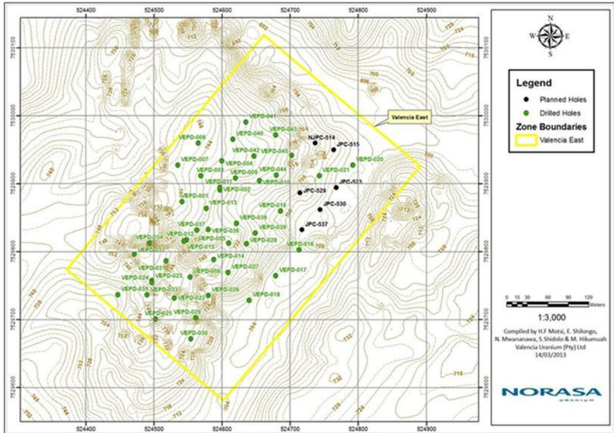
FIGURE 2a. Surface topography of Valencia East
