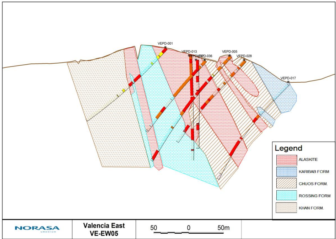
FIGURE 3. Valencia E Section Line 5 EW, with D-type alaskite in the Damara Metasediment succession.
