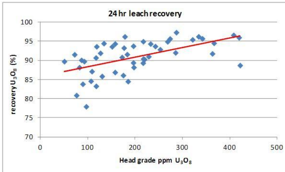
FIGURE 5. Distribution of recoveries as a function of grade after 24hrs.
