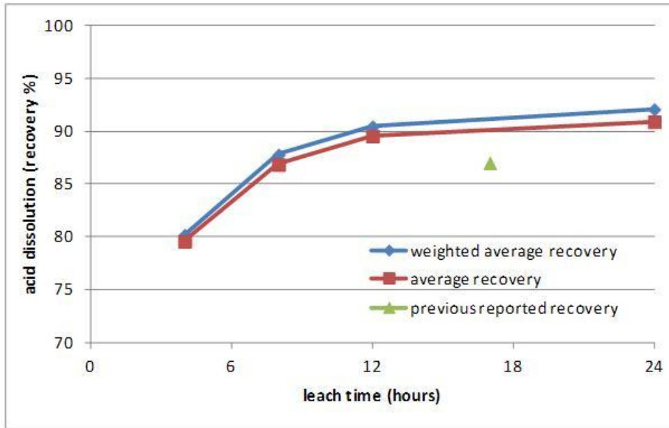
FIGURE 7. Leach recovery performance - overall average.
