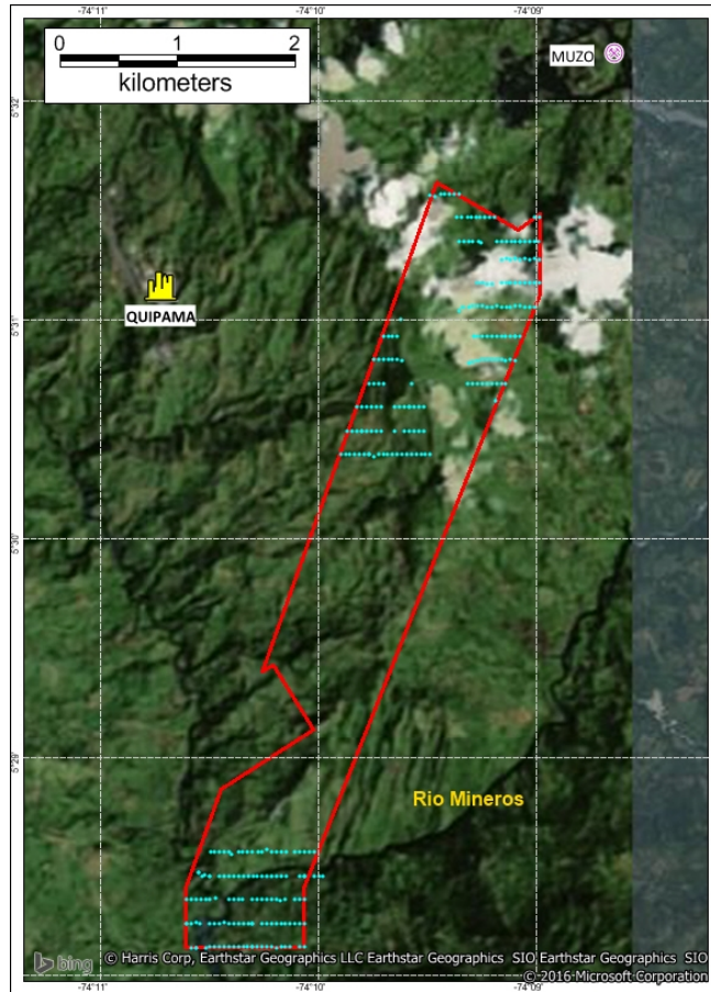
Figure 2: Map showing the collection points in blue, carried out in a grid 200x40m. Only in the central part of the North Area was it not possible to collect due to extremely steep relief.
