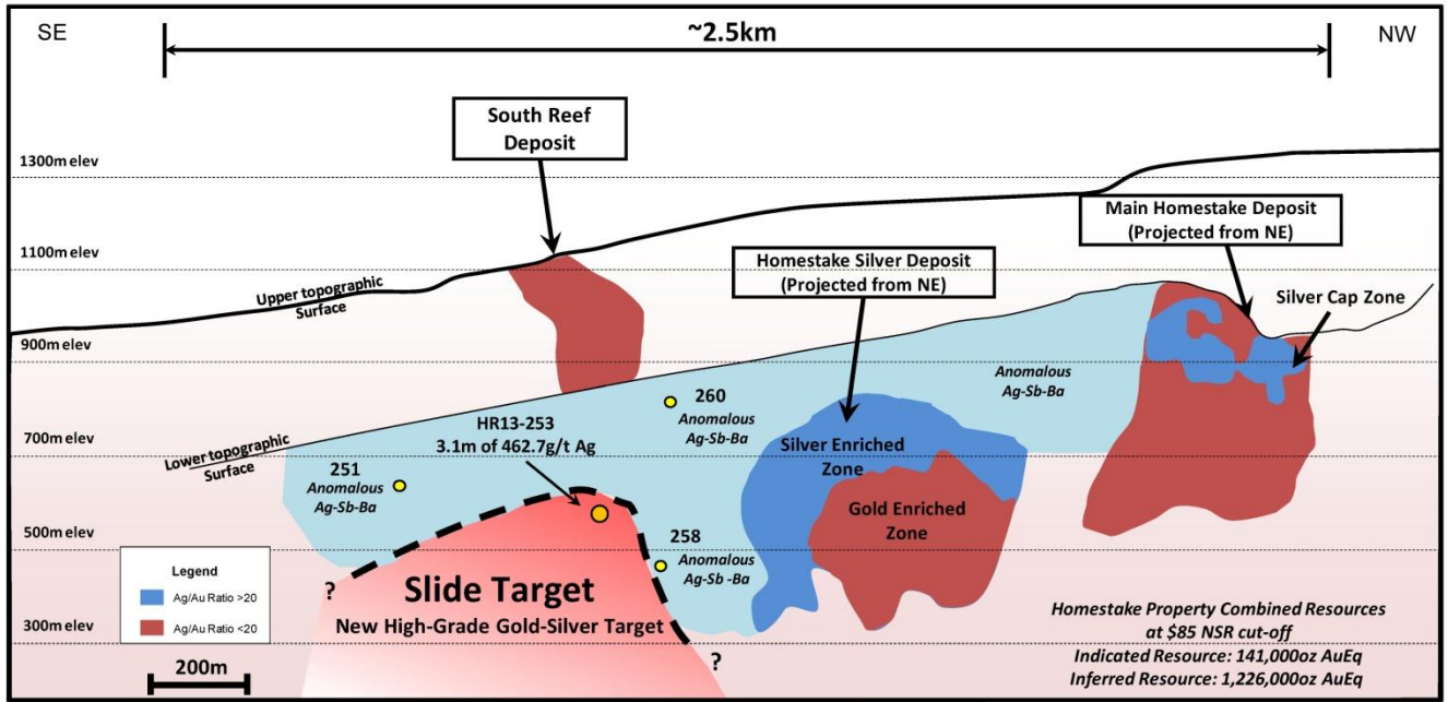
Figure 1: Longitudinal section showing Slide target at Homestake Ridge property.
