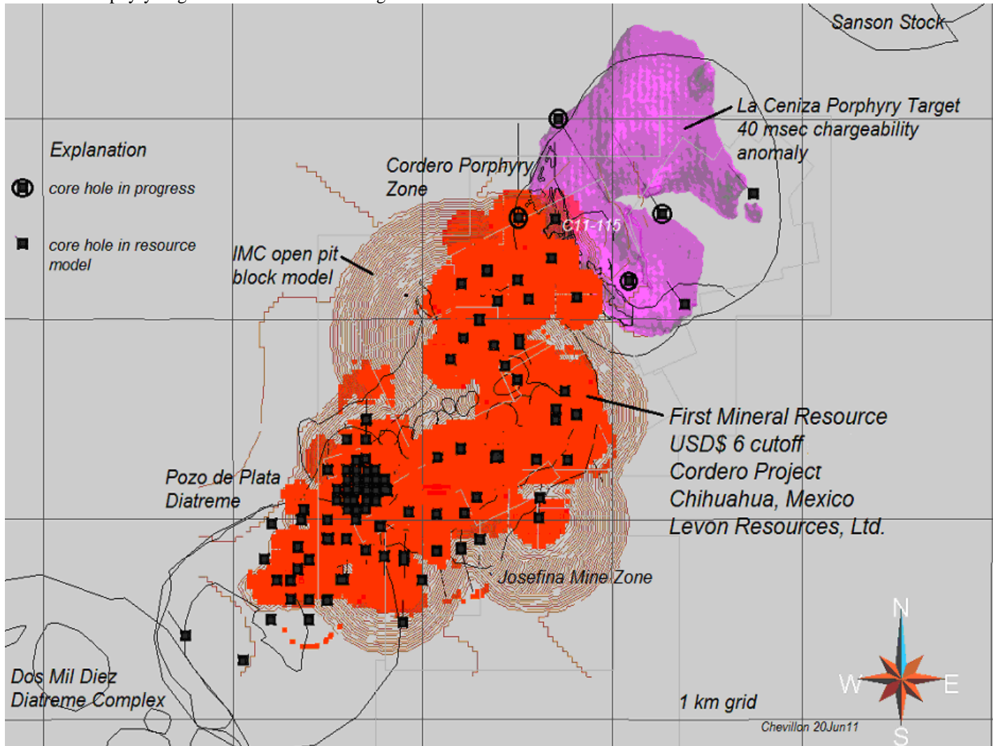
Figure 1. Map of the first Cordero mineral resource, the core holes in the model, the IMC modeled open pit and the La Ceniza Porphyry target with current holes being drilled.
