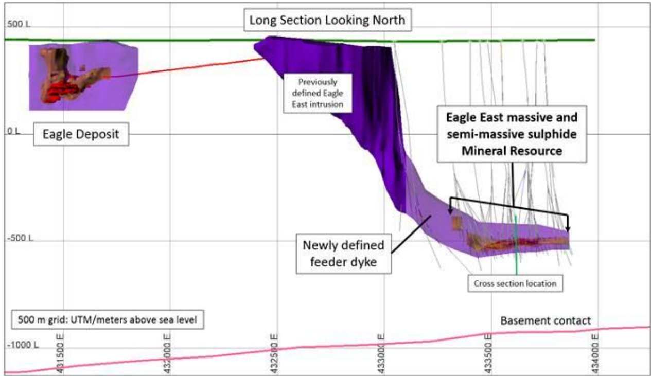
Figure 1 – Eagle and Eagle East long section showing exploration drill hole traces and an outline of the Eagle East mineralization.
