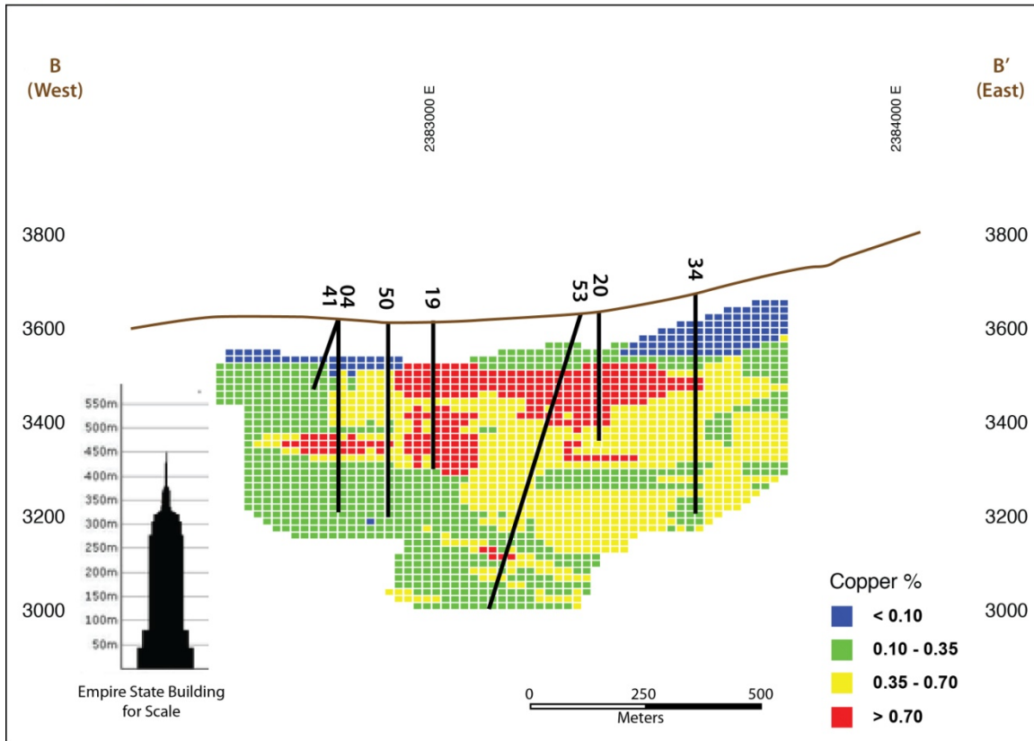
Figure 3 – Cross Section Map
