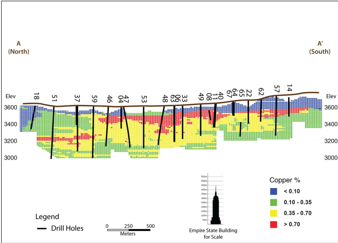
Figure 2 –Vertical Longitudinal Map
