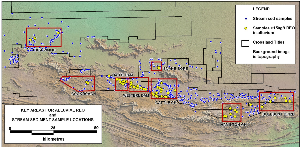
Figure 1 - Shows locations of stream sediment samples, Samples >150g/t REO and Key Areas for further work
