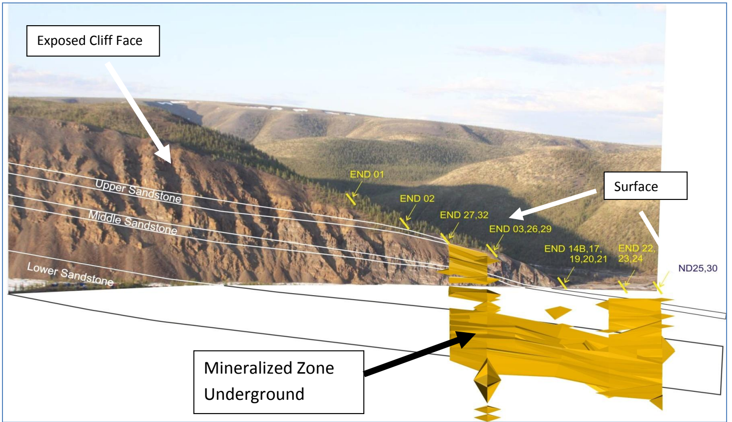
Figure 1 - Volume interpretation of Nizhny Endybal prospect area (in yellow) looking south east (not to scale)
