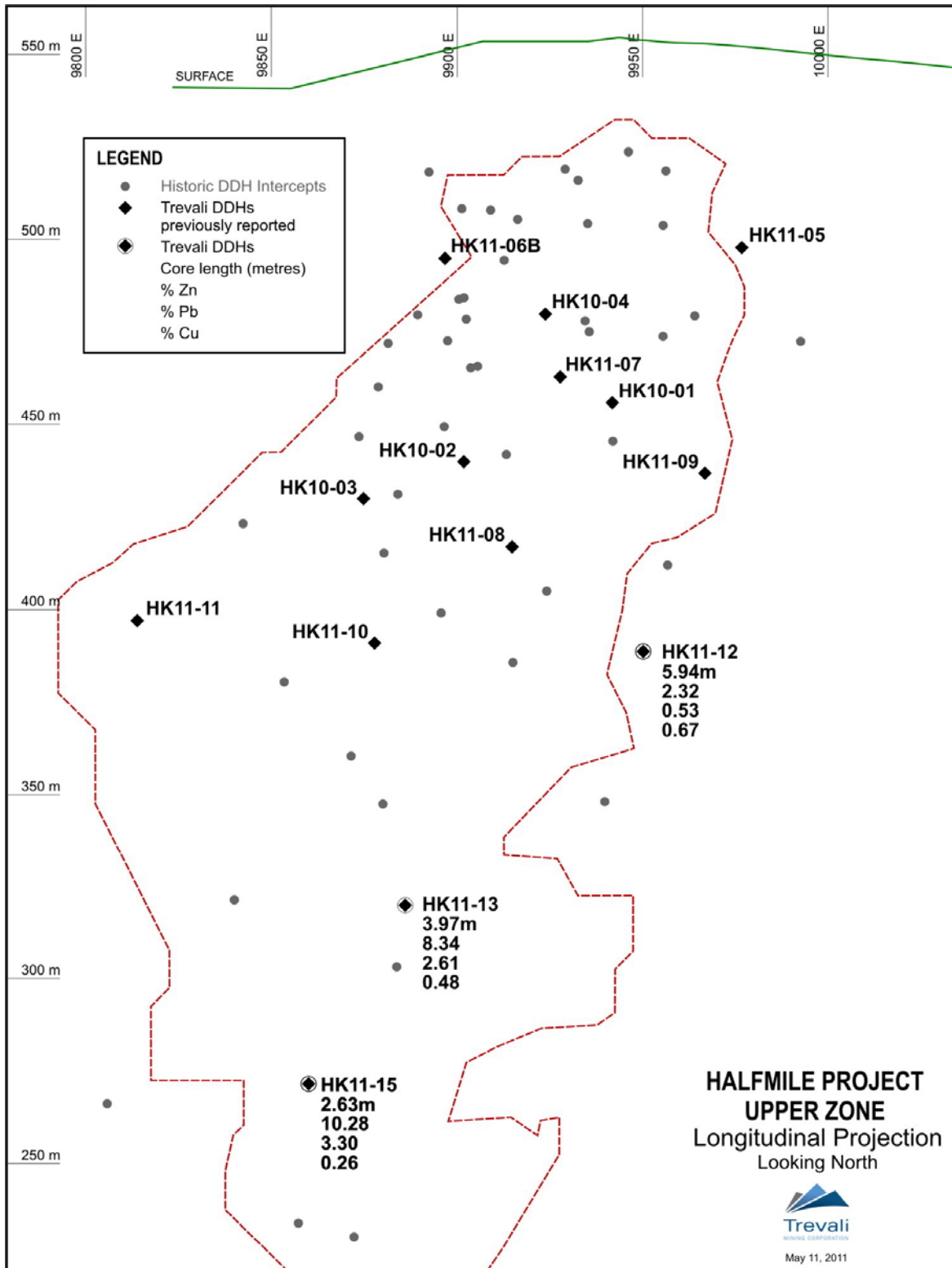
Figure 1. Longitudinal projection of Upper Zone of Halfmile Deposit
