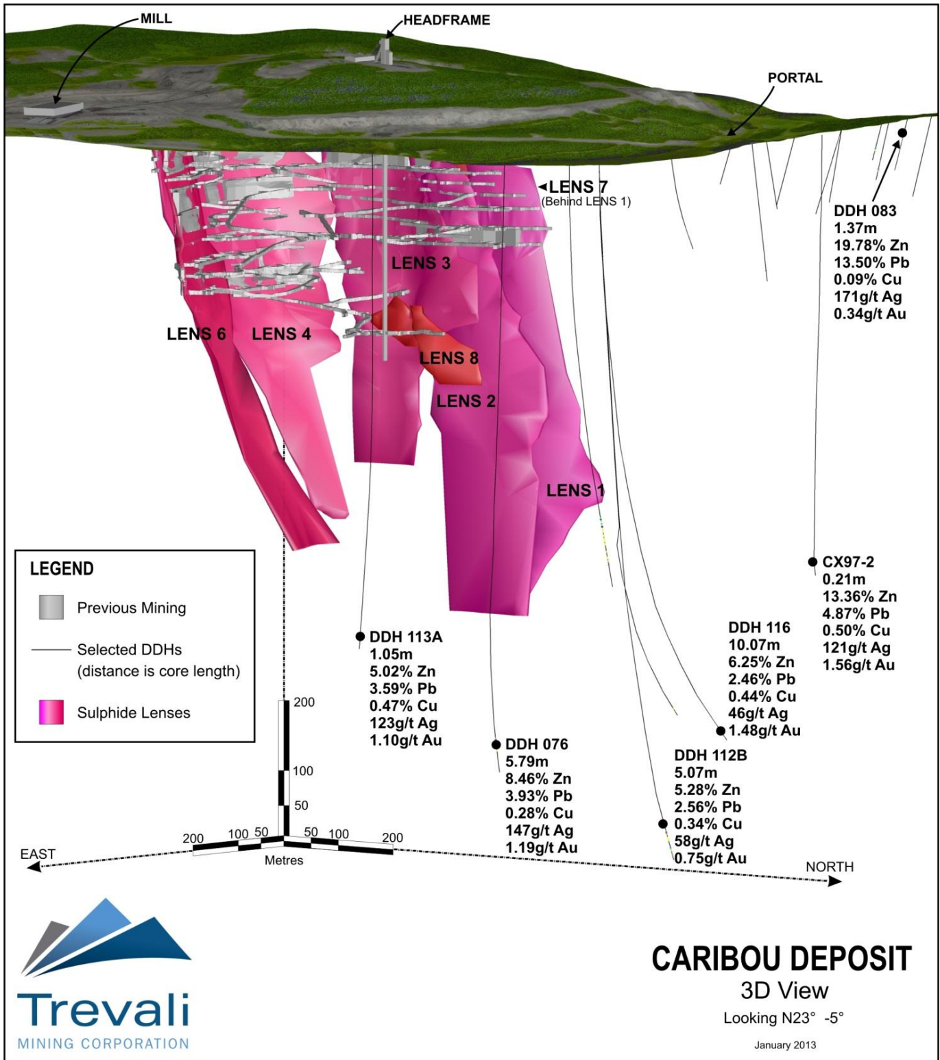
Figure 1: Three-dimensional view of the Caribou Deposit, in New Brunswick’s Bathurst Mining Camp, showing location of the extensive existing surface and underground infrastructure, various mineralized lenses and significant drill-hole intercepts located outside of the current resource estimate.
