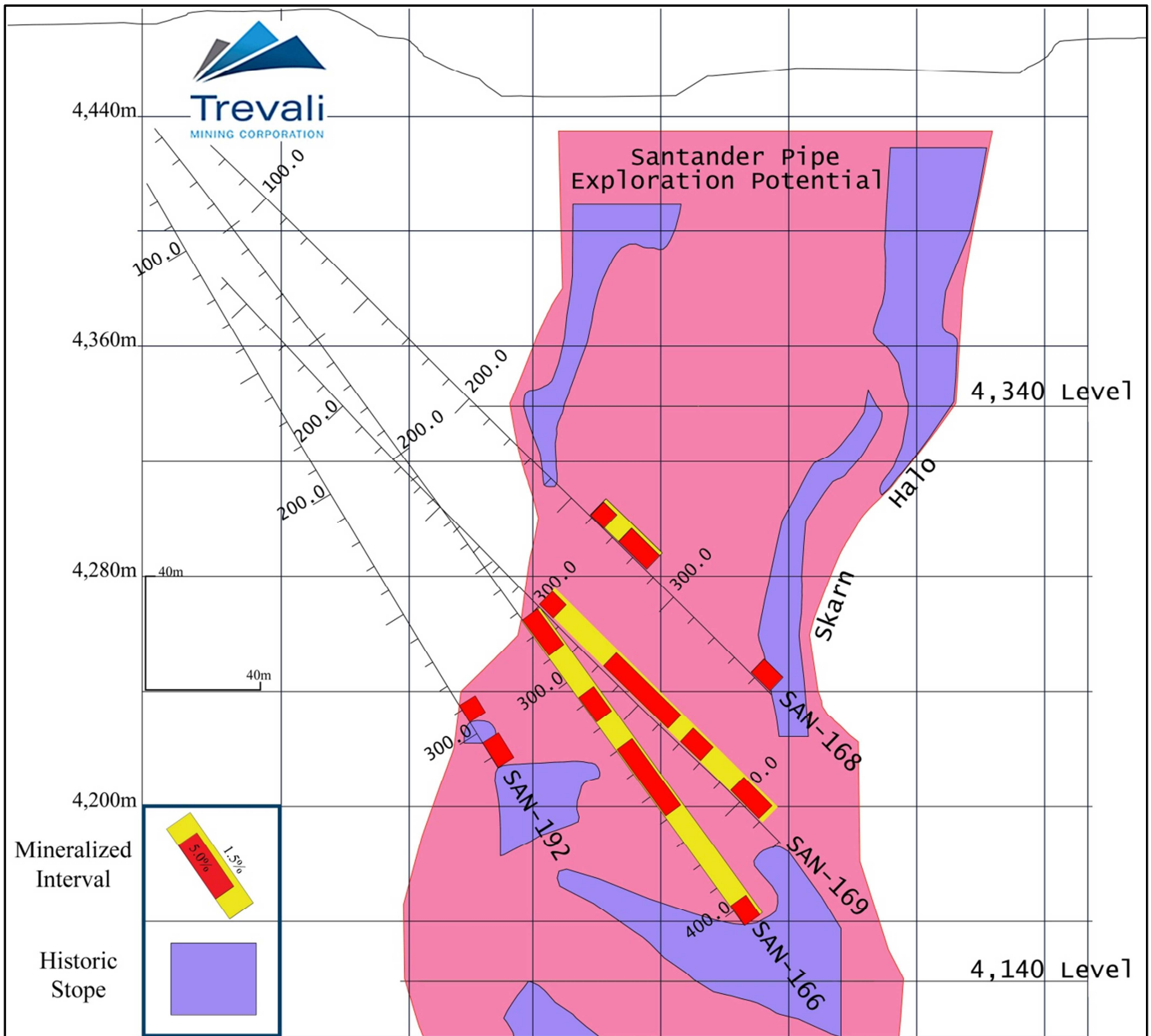
Figure 1: N-S cross section of the former producing Santander Pipe.
