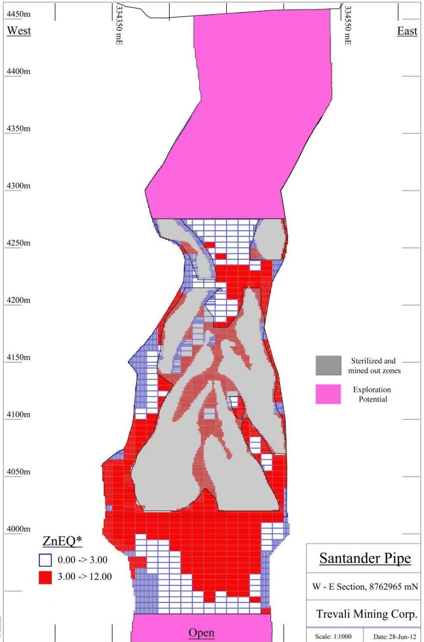
Figure 4: Santander Pipe Section Looking North.
